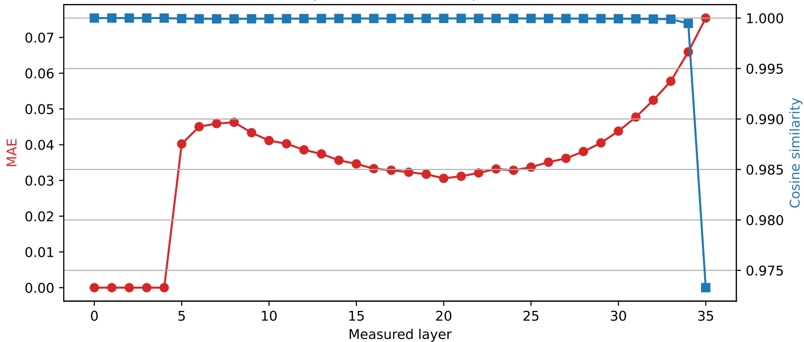
SmolLM3-3B | Quantized layer 4 | float64 \rightarrow int2
