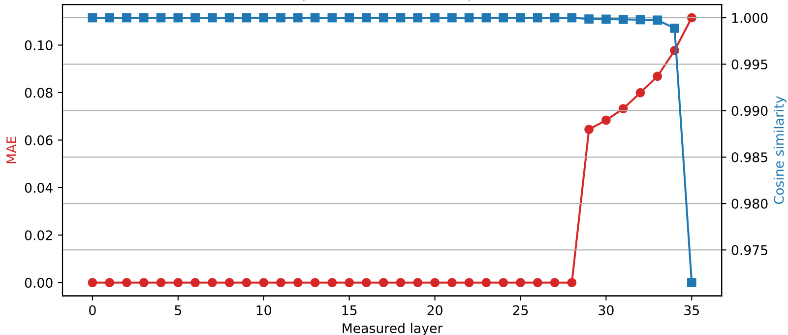
SmolLM3-3B | Quantized layer 28 | float64 → int2
