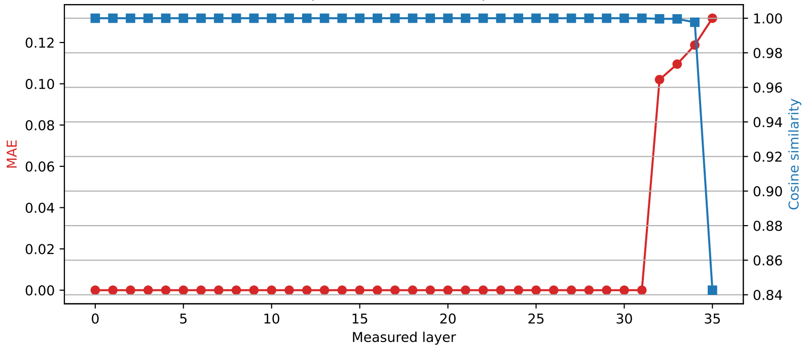
SmolLM3-3B | Quantized layer 31 | float64 \rightarrow int2
