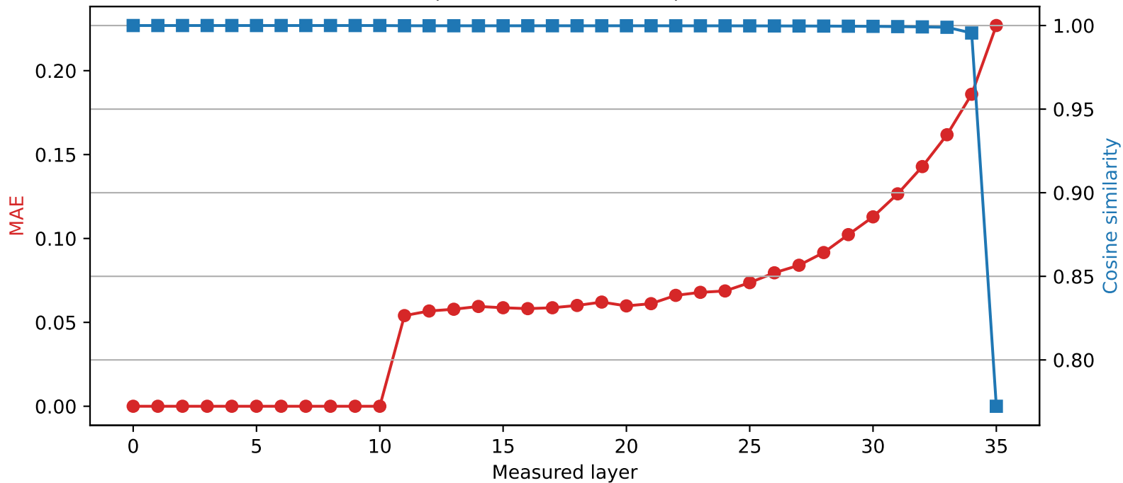
SmolLM3-3B | Quantized layer 10 | float64 \rightarrow int2
