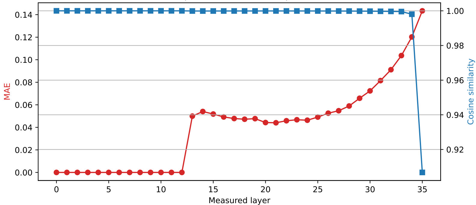
SmolLM3-3B | Quantized layer 12 | float64 → int2
