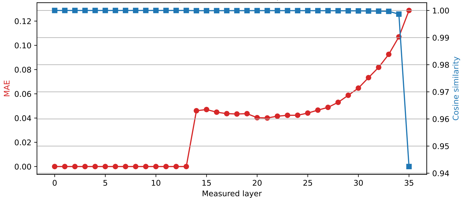
SmolLM3-3B | Quantized layer 13 | float64 → int2
