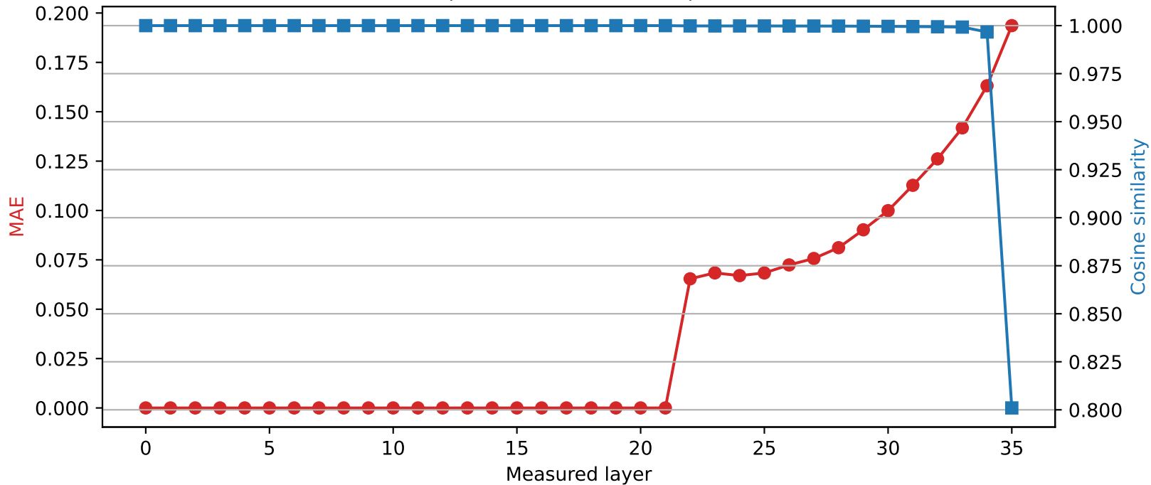
SmolLM3-3B | Quantized layer 21 | float64 → int2
