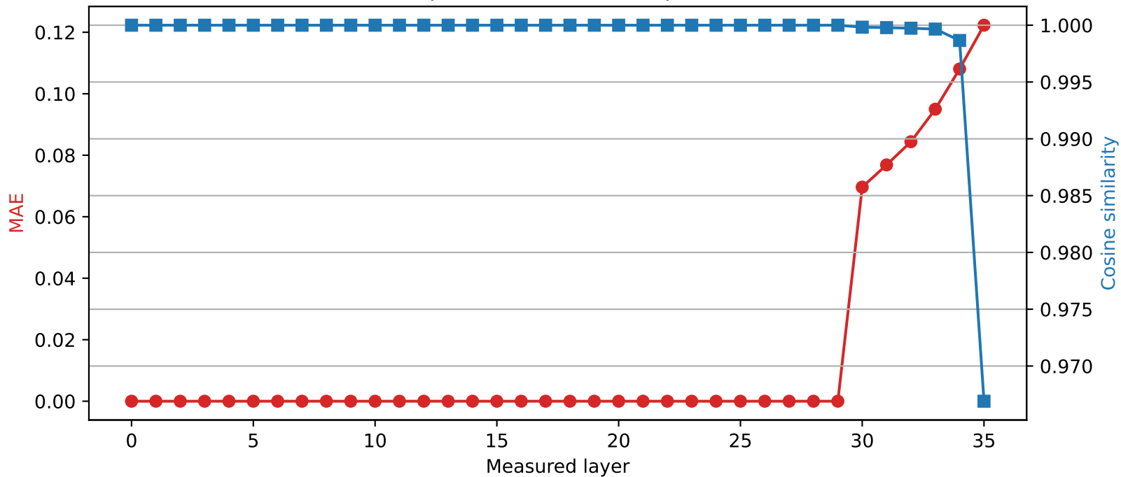
SmolLM3-3B | Quantized layer 29 | float64 → int2
