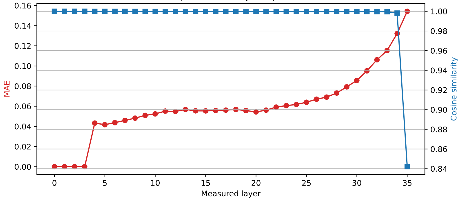
SmolLM3-3B | Quantized layer 3 | float64 \rightarrow int2
