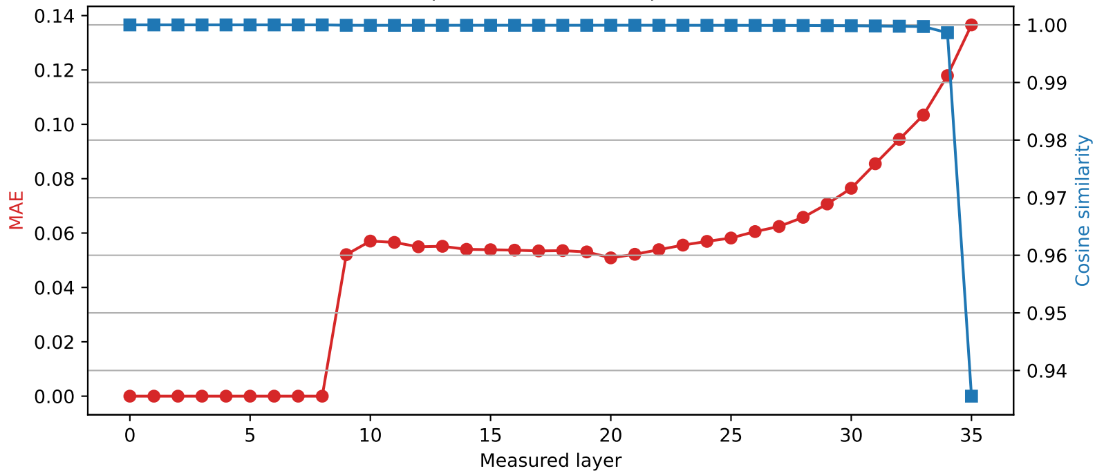
SmolLM3-3B | Quantized layer 8 | float64 → int2
