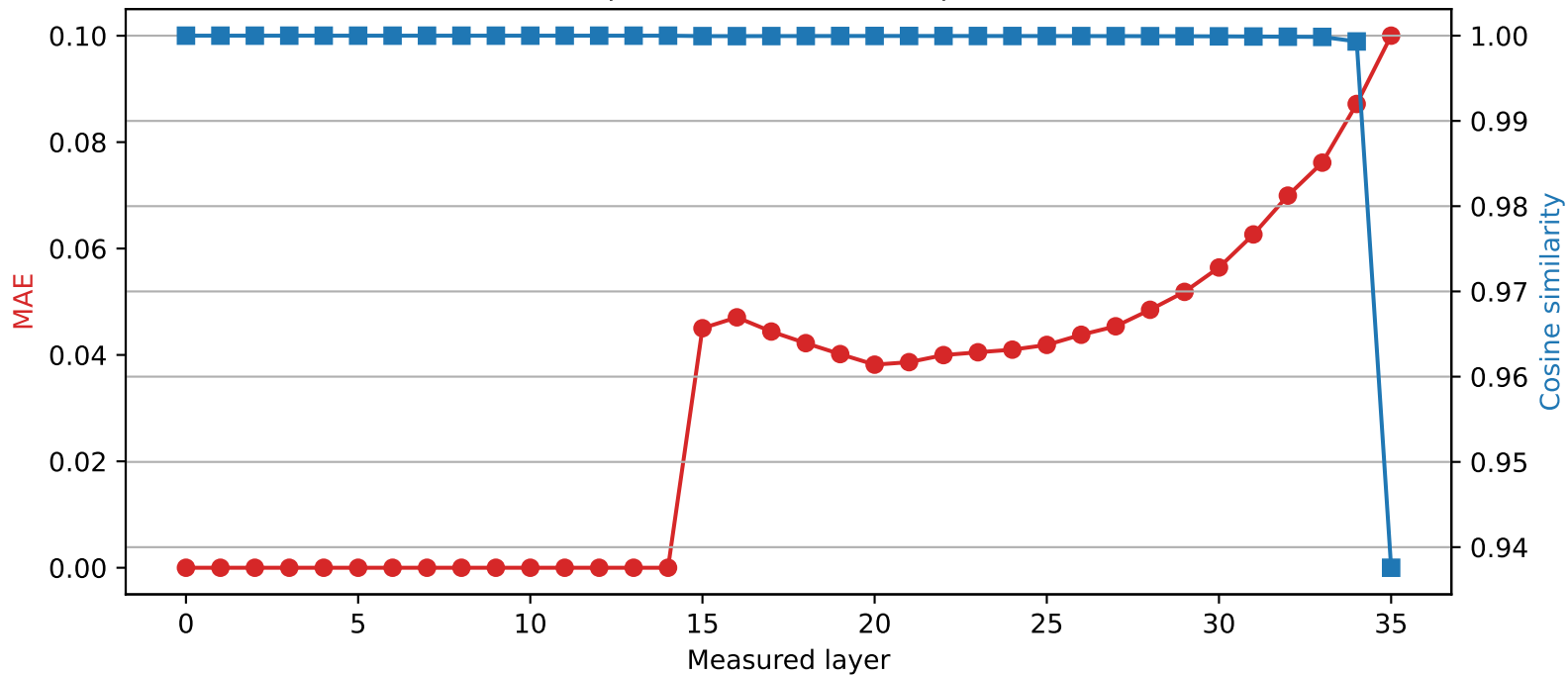
SmolLM3-3B | Quantized layer 14 | float64 → int2
