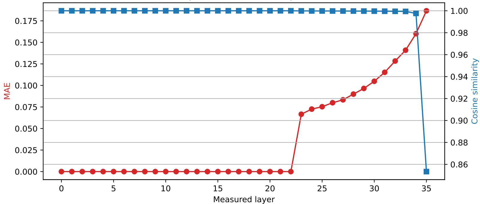
SmolLM3-3B | Quantized layer 22 | float64 → int2
