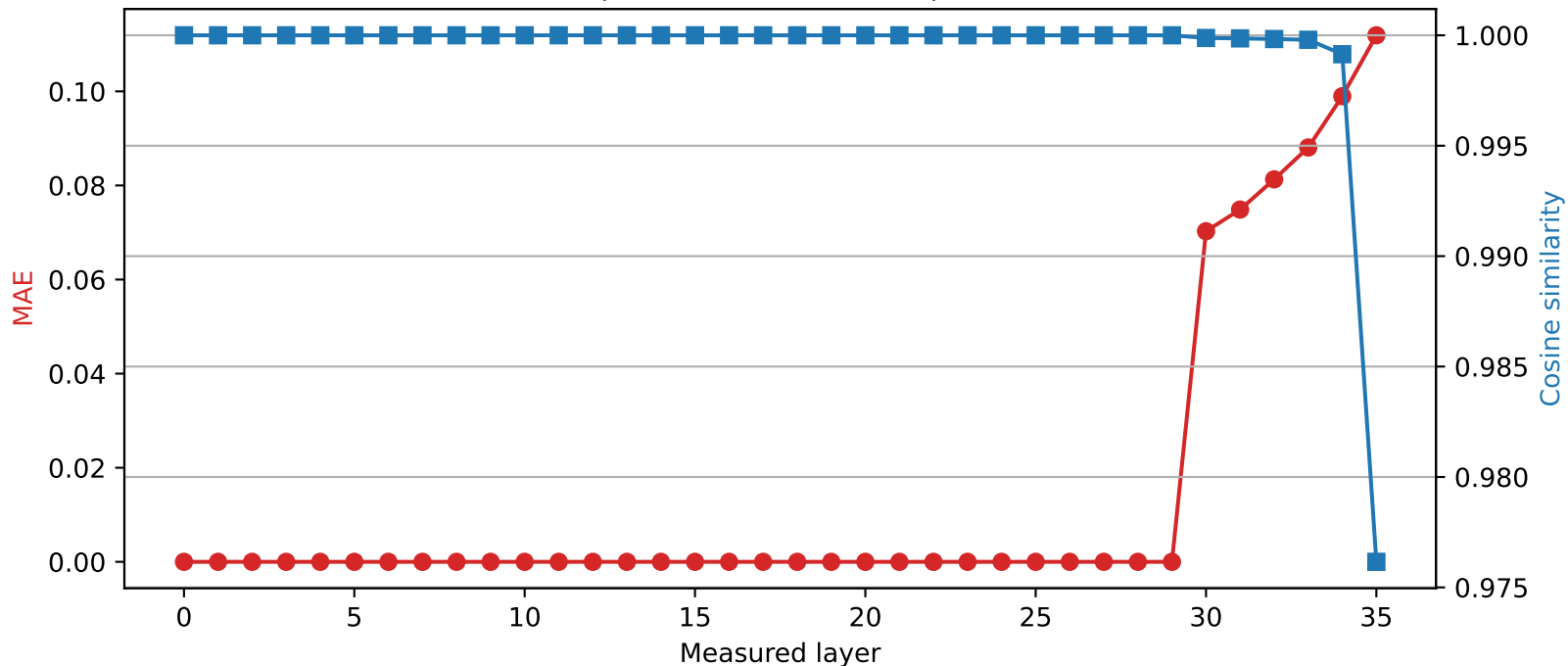
SmolLM3-3B | Quantized layer 29 | float64 \rightarrow int2
