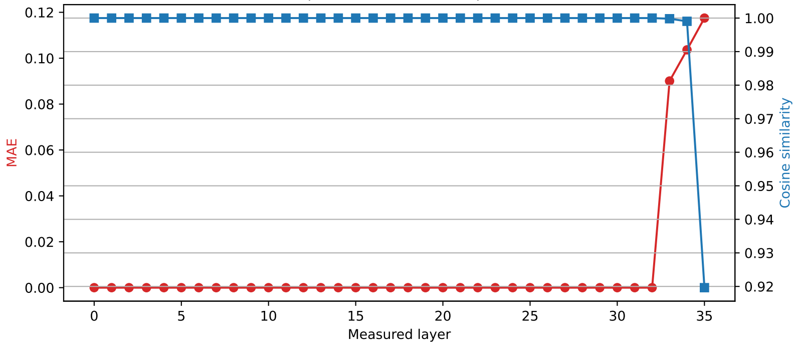
SmolLM3-3B | Quantized layer 32 | float64 \rightarrow int2
