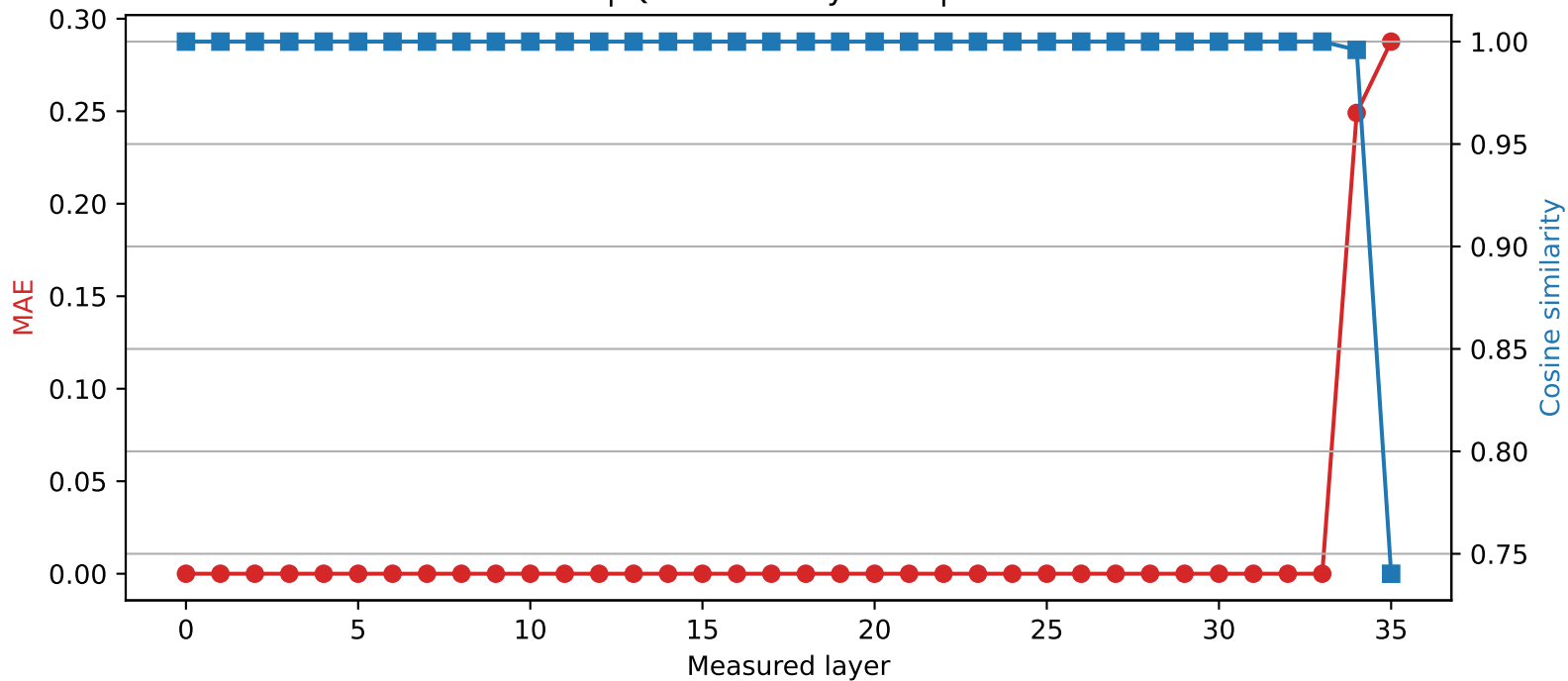
SmolLM3-3B | Quantized layer 33 | float64 → int2
