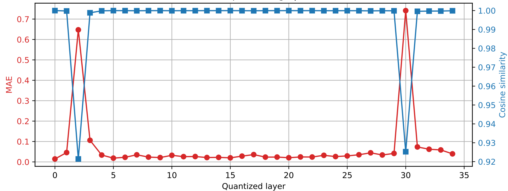
Qwen2.5-3B | Prompt 0 Final RMSNorm output damage | float16 \rightarrow int8
