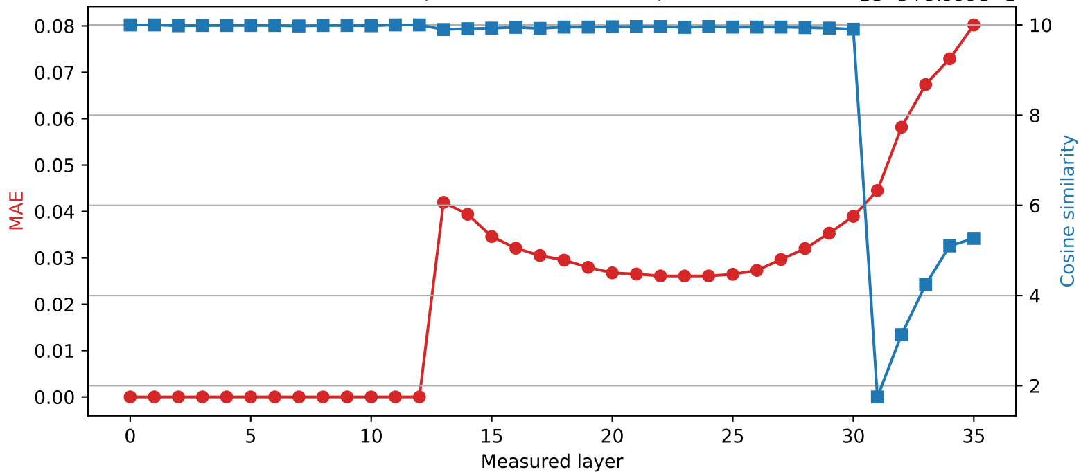
Qwen2.5-3B | Quantized layer 12 | float16 → int8
