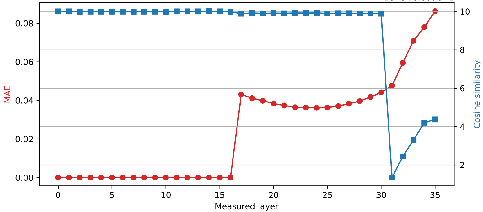
Qwen2.5-3B | Quantized layer 16 | float16 → int8
