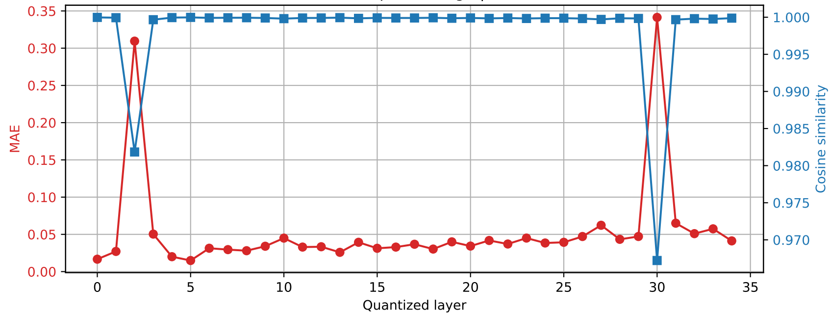
Qwen2.5-3B | Prompt 1 Final RMSNorm output damage | float16 \rightarrow int8
