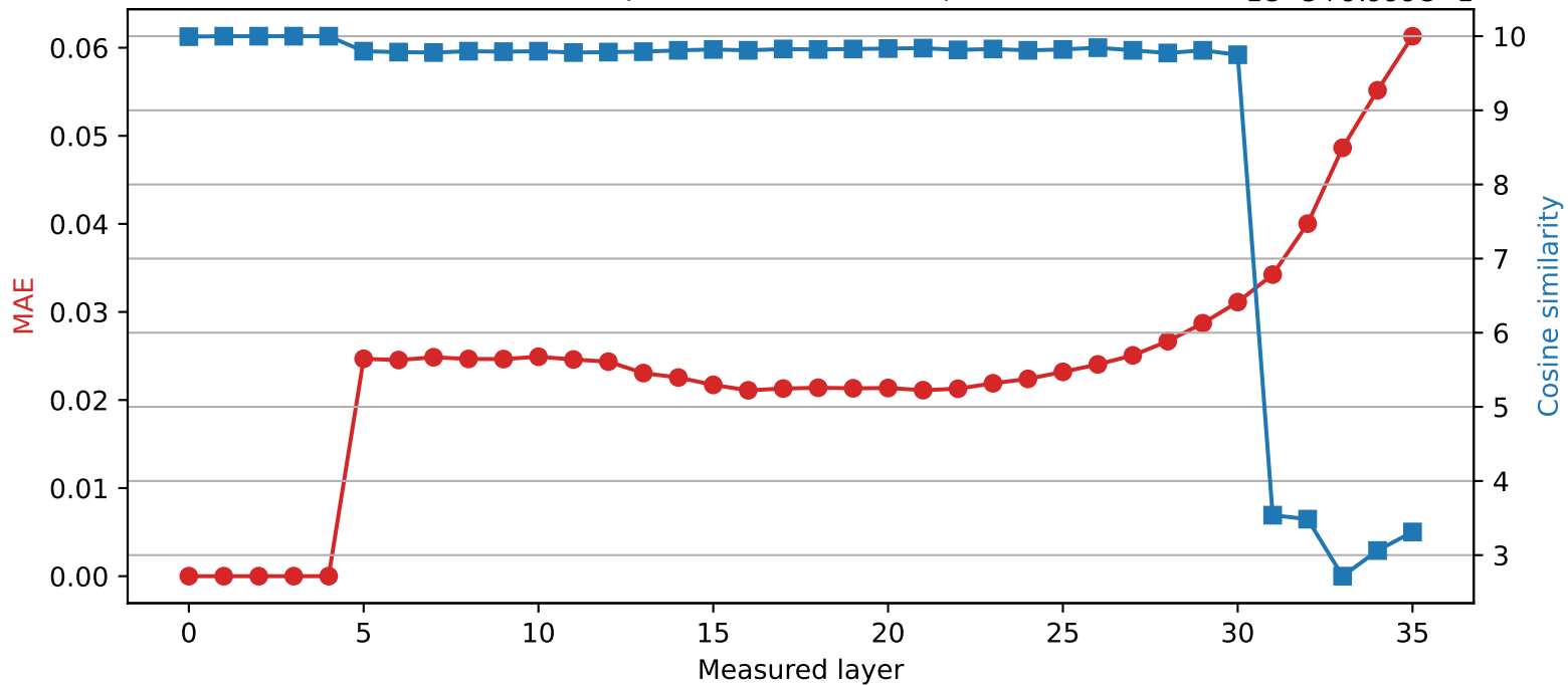
Qwen2.5-3B | Quantized layer 4 | float16 → int8
