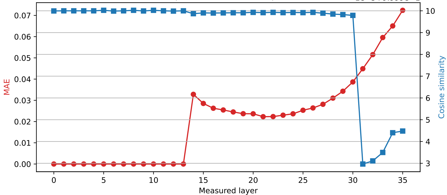
Qwen2.5-3B | Quantized layer 13 | float16 → int8
