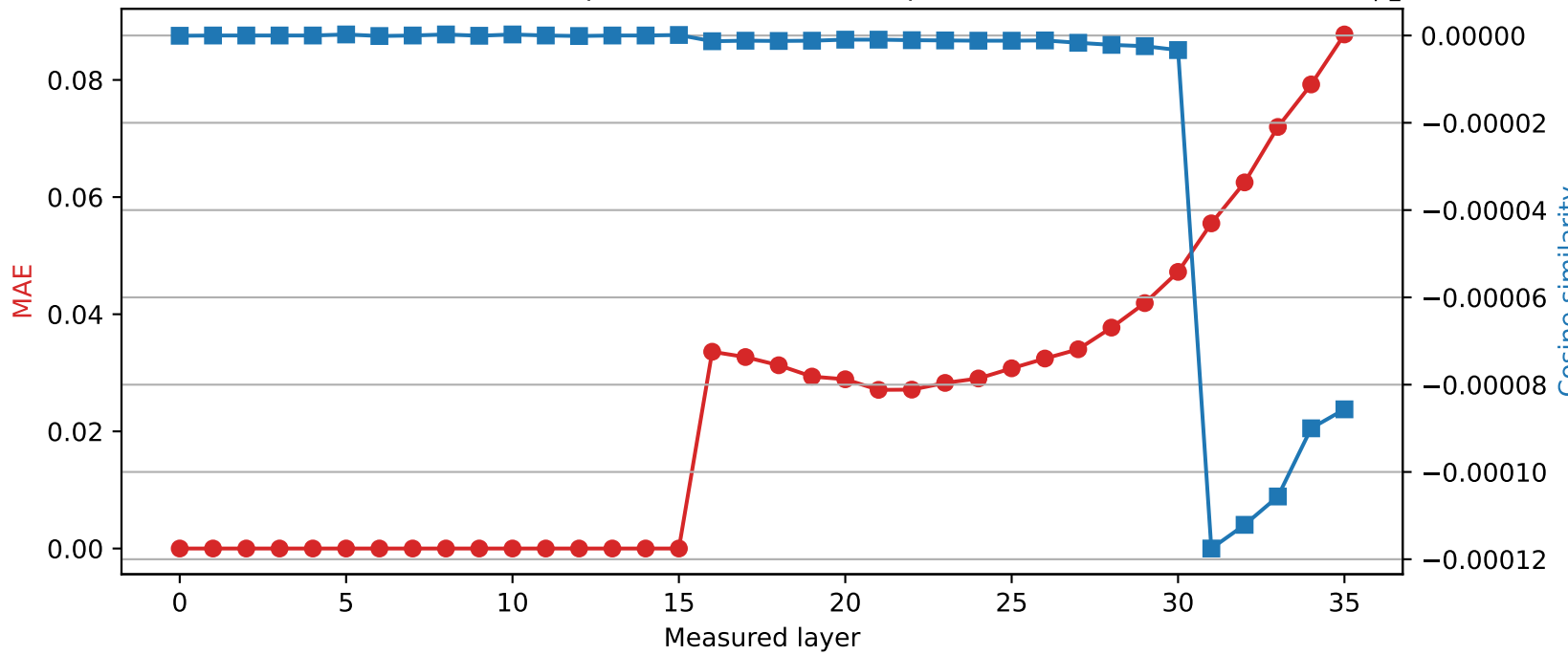
Qwen2.5-3B | Quantized layer 15 | float16 → int8
