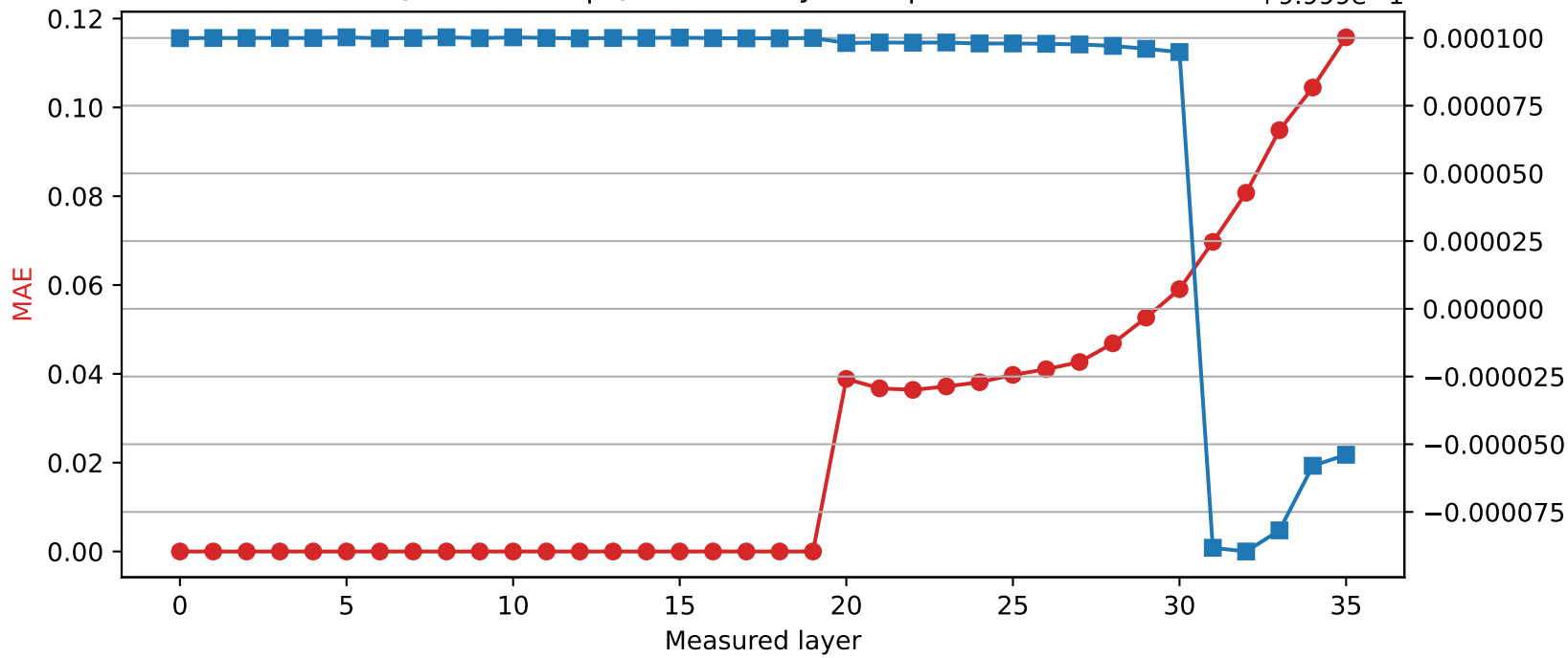
Qwen2.5-3B | Quantized layer 19 | float16 → int8
