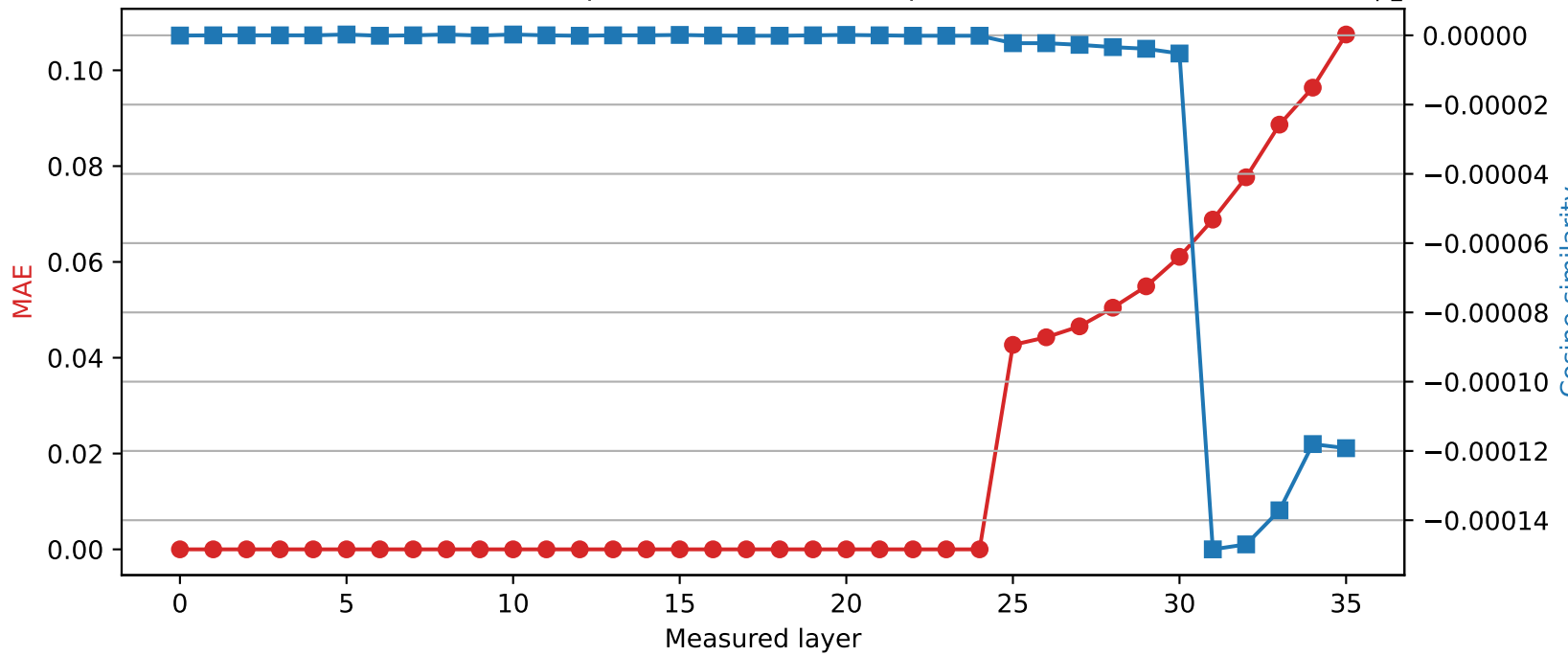
Qwen2.5-3B | Quantized layer 24 | float16 → int8
