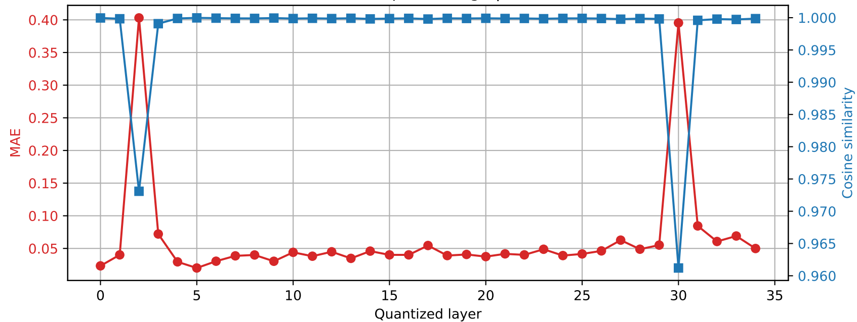
Qwen2.5-3B | Prompt 2 Final RMSNorm output damage | float16 \rightarrow int8
