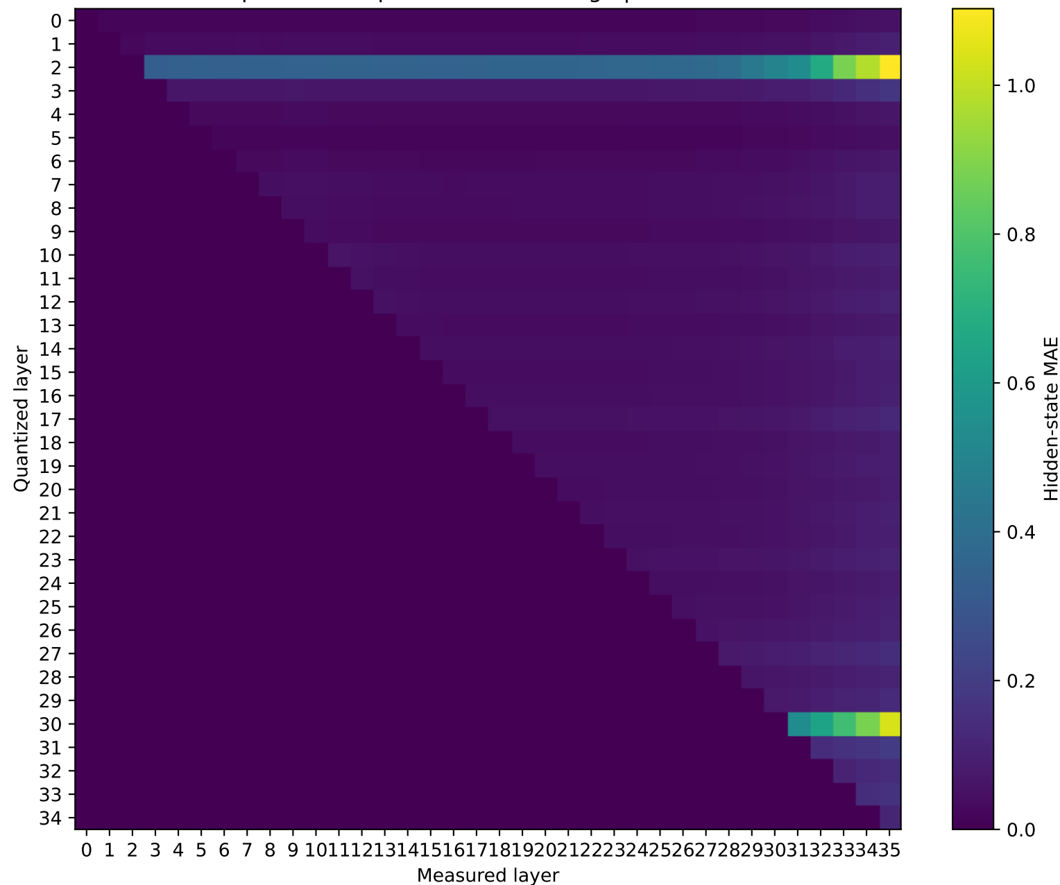
Qwen2.5-3B Prompt 2: MAE representation damage | float16 → int8
