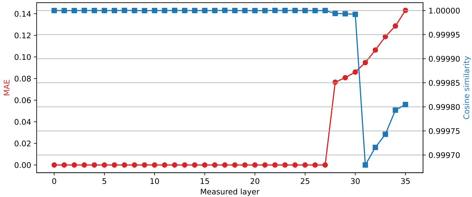
Qwen2.5-3B | Quantized layer 27 | float16 → int8
