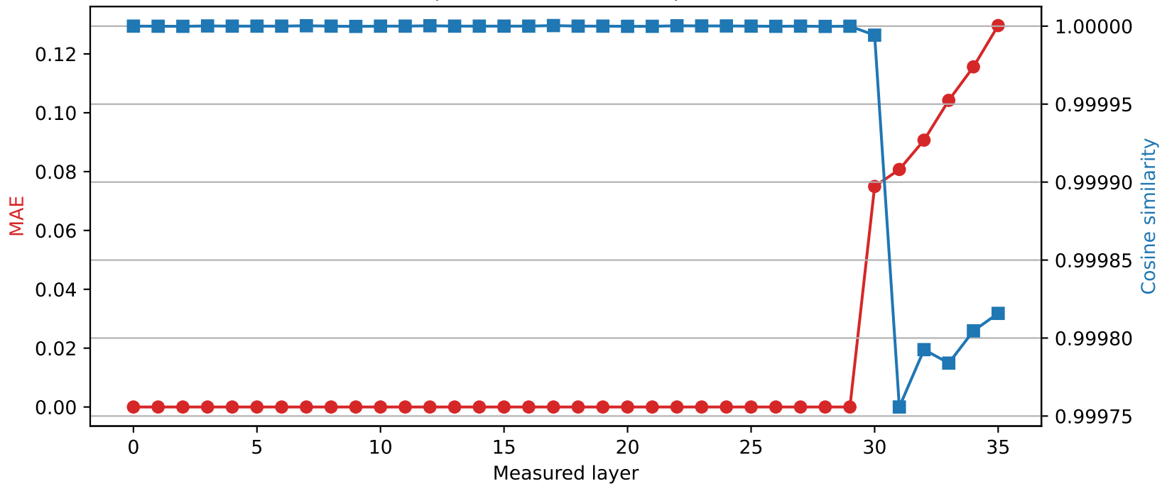
Qwen2.5-3B | Quantized layer 29 | float16 \rightarrow int8
