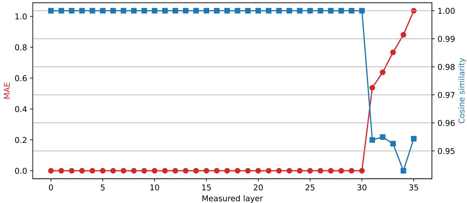
Qwen2.5-3B | Quantized layer 30 | float16 \rightarrow int8
