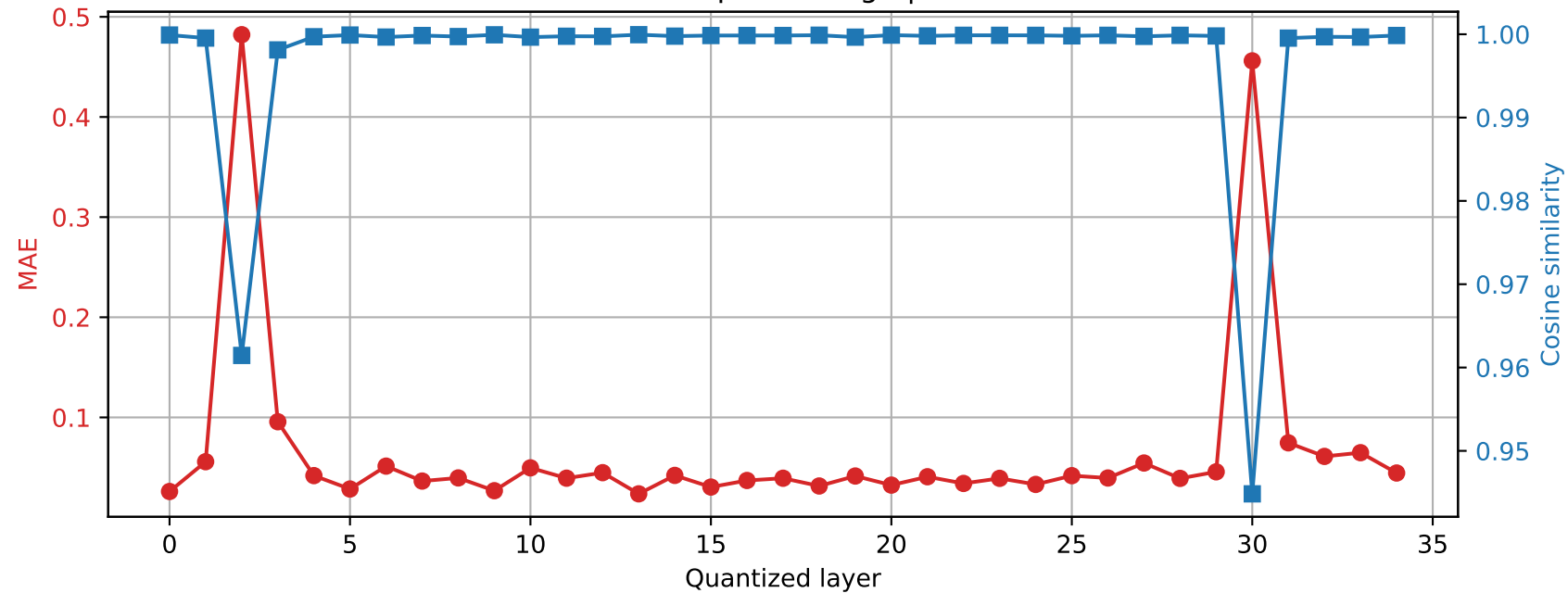
Qwen2.5-3B | Prompt 3 Final RMSNorm output damage | float16 \rightarrow int8
