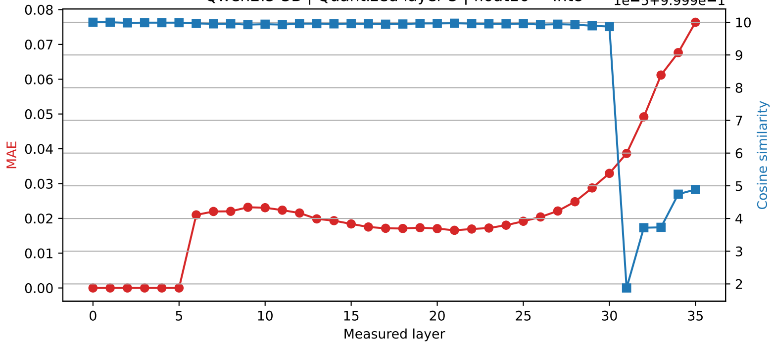
Qwen2.5-3B | Quantized layer 5 | float16 → int8
