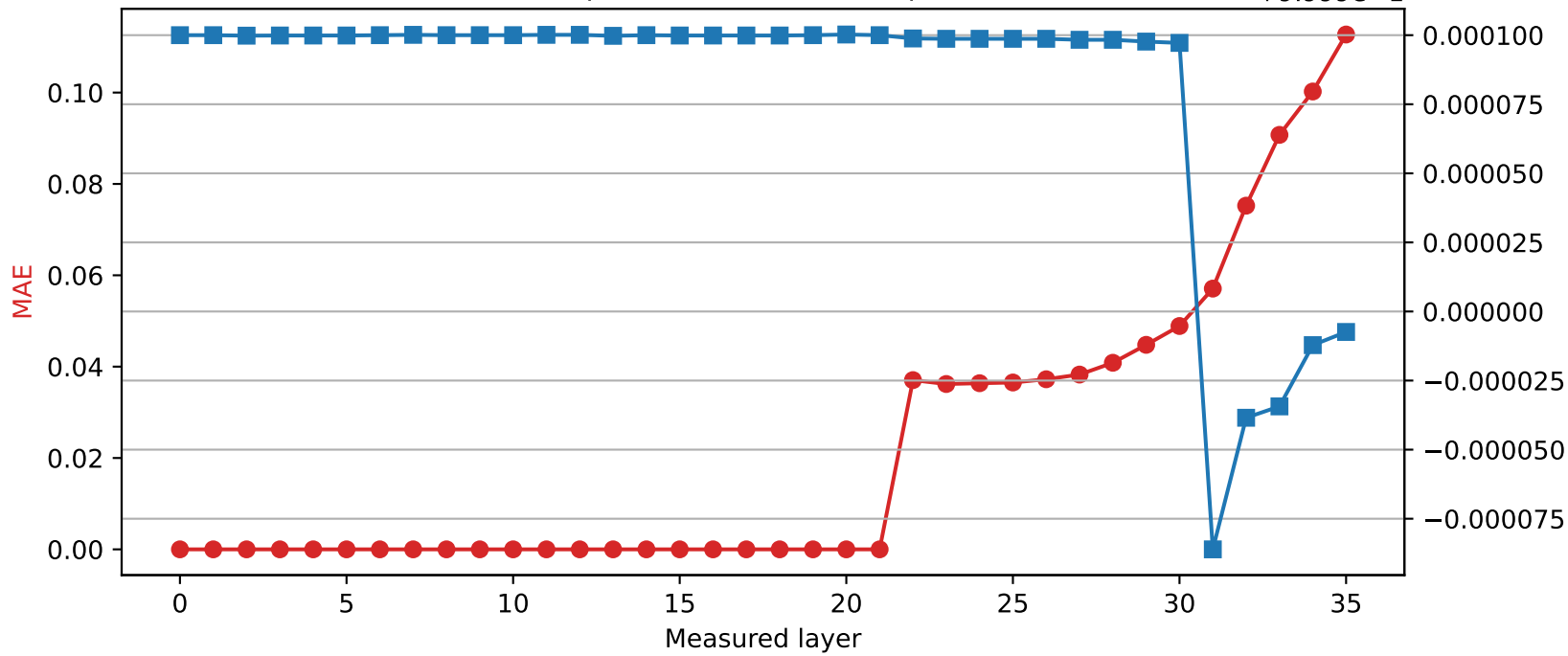
Qwen2.5-3B | Quantized layer 21 | float16 → int8
