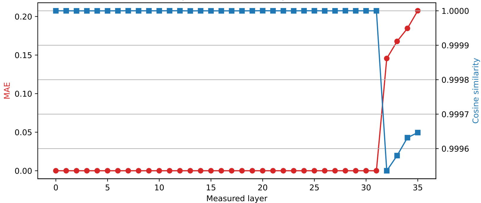
Qwen2.5-3B | Quantized layer 31 | float16 \rightarrow int8
