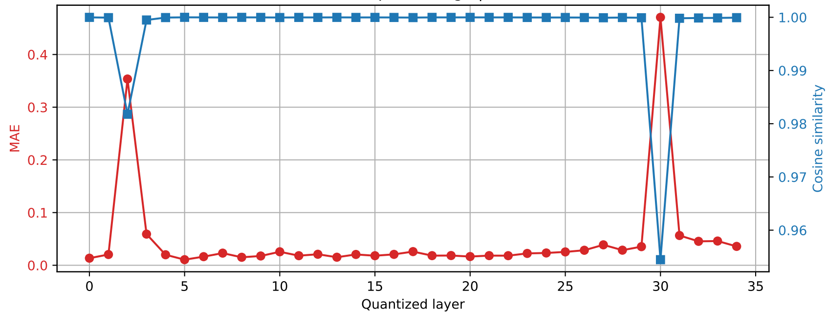
Qwen2.5-3B | Prompt 4 Final RMSNorm output damage | float16 \rightarrow int8
