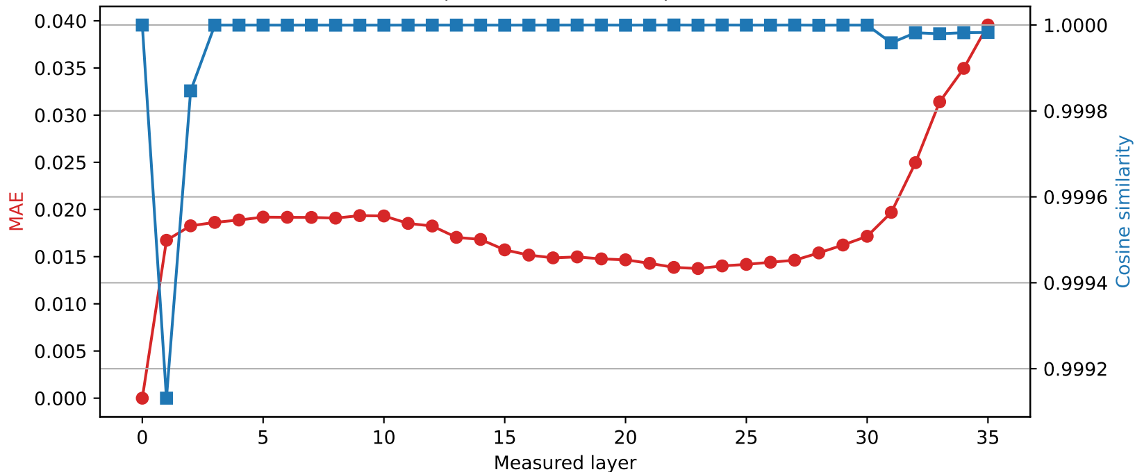
Qwen2.5-3B | Quantized layer 0 | float16 \rightarrow int8
