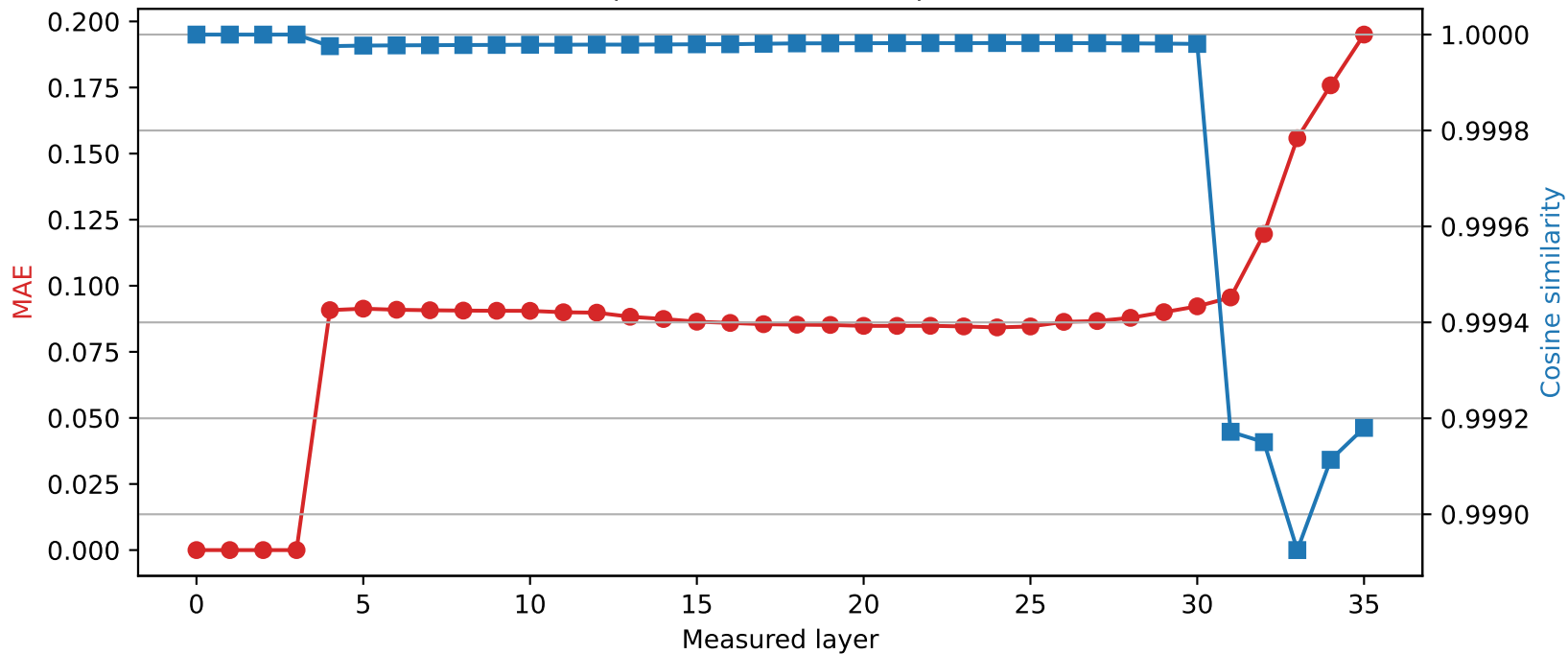
Qwen2.5-3B | Quantized layer 3 | float16 → int8
