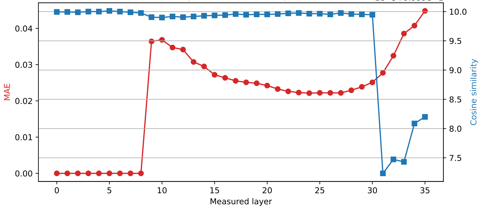
Qwen2.5-3B | Quantized layer 8 | float16 → int8
