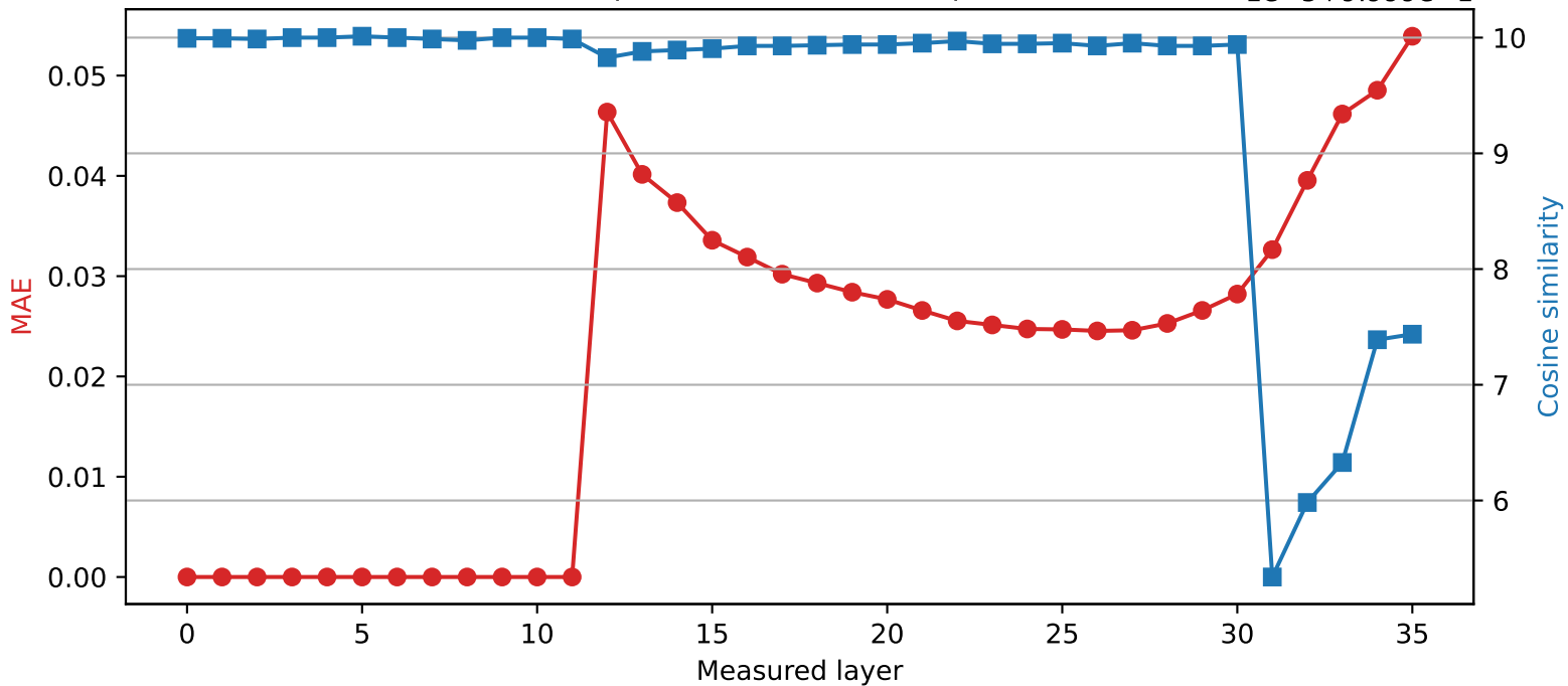
Qwen2.5-3B | Quantized layer 11 | float16 → int8
