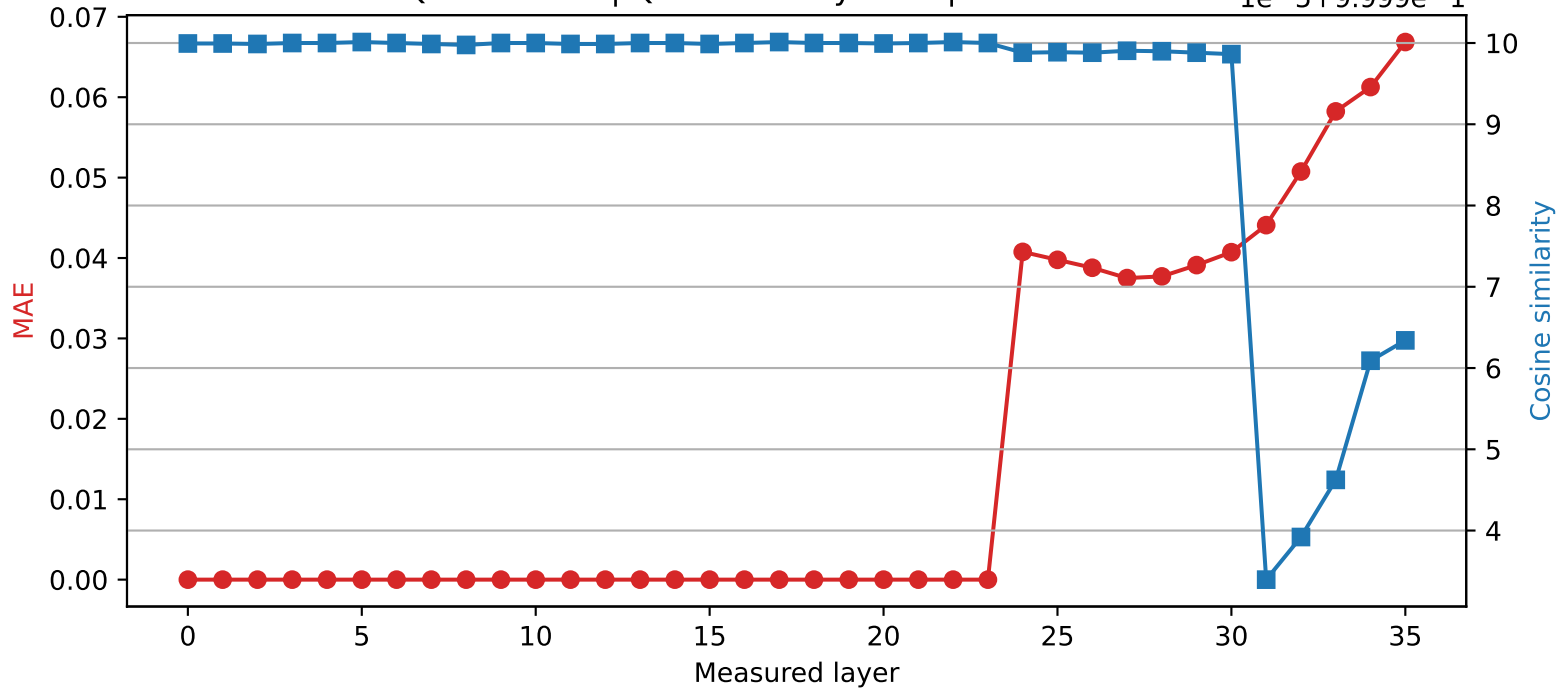
Qwen2.5-3B | Quantized layer 23 | float16 → int8
