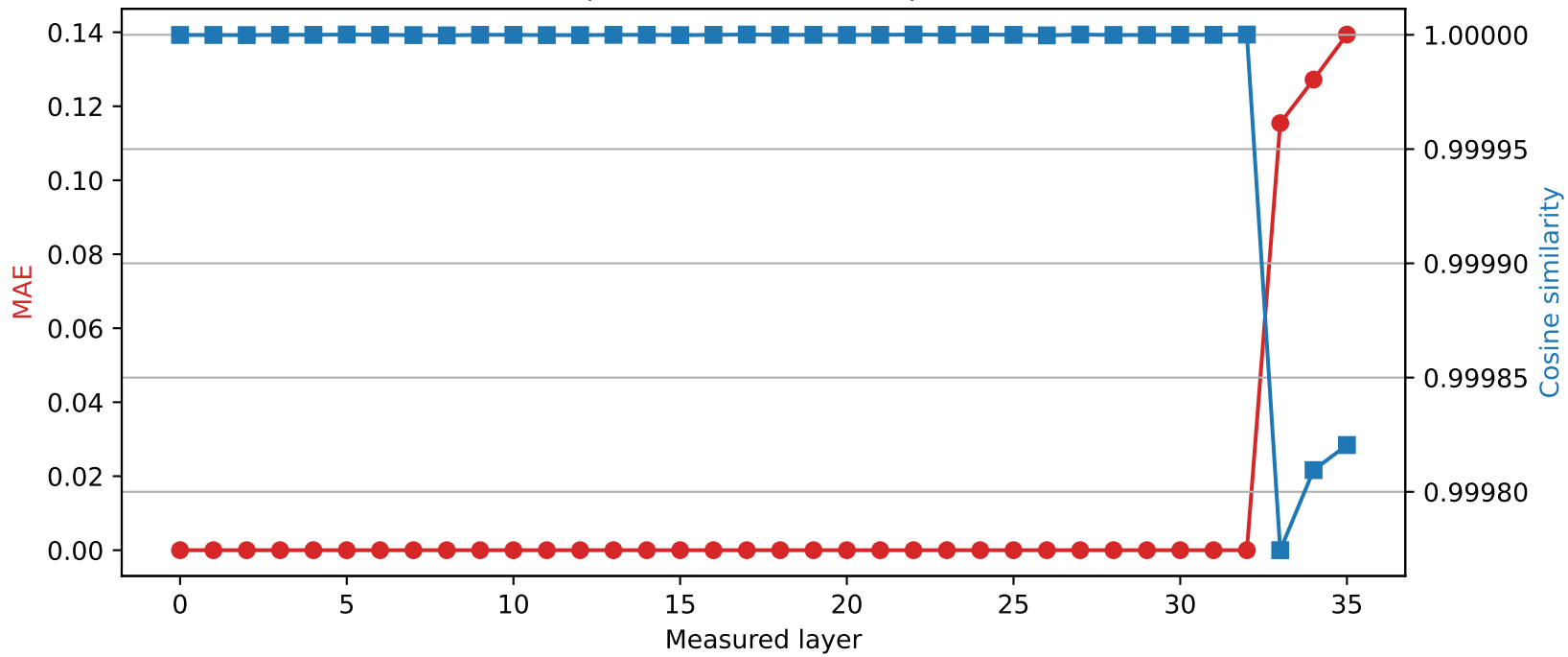
Qwen2.5-3B | Quantized layer 32 | float16 \rightarrow int8
