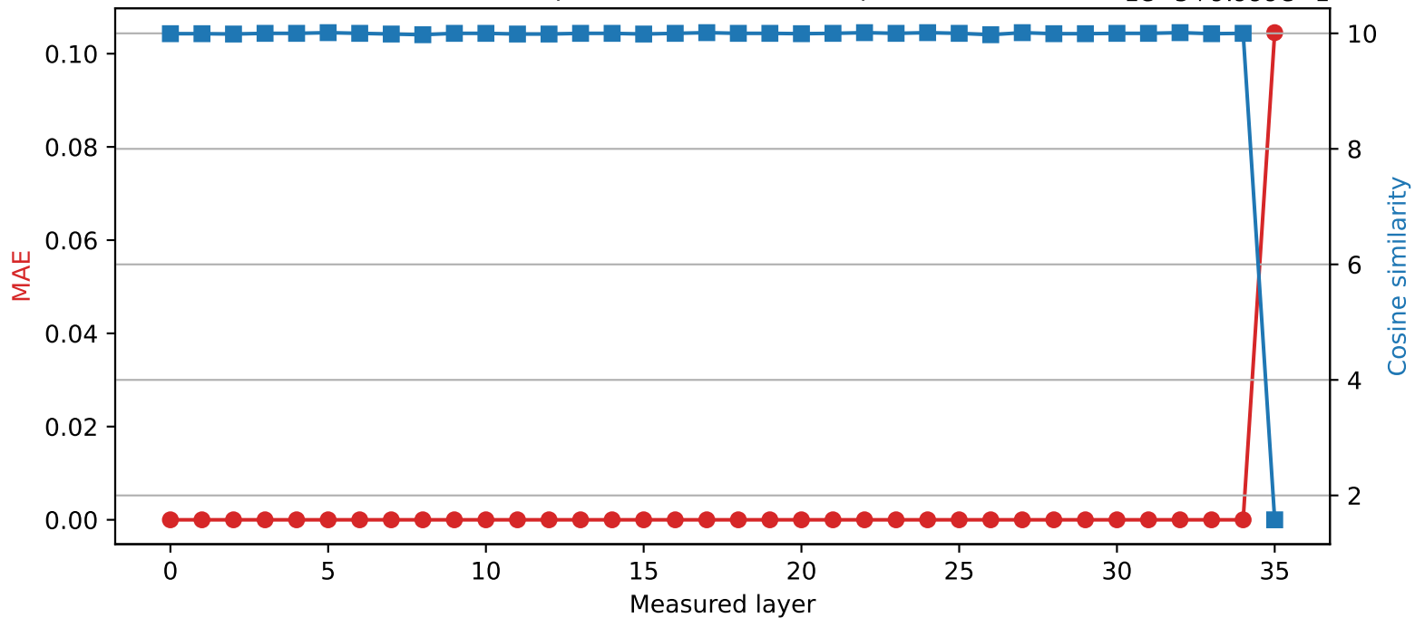
Qwen2.5-3B | Quantized layer 34 | float16 → int8
