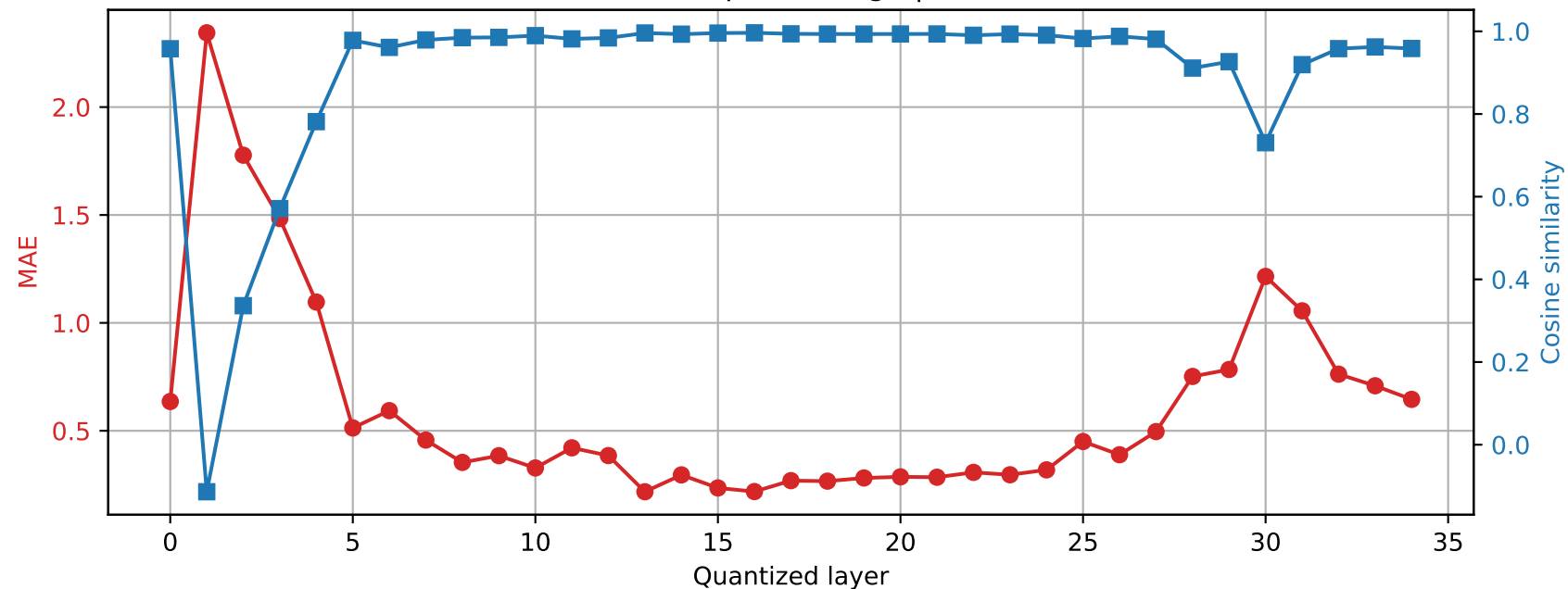
Qwen2.5-3B | Prompt 0 Final RMSNorm output damage | float16 \rightarrow int4
