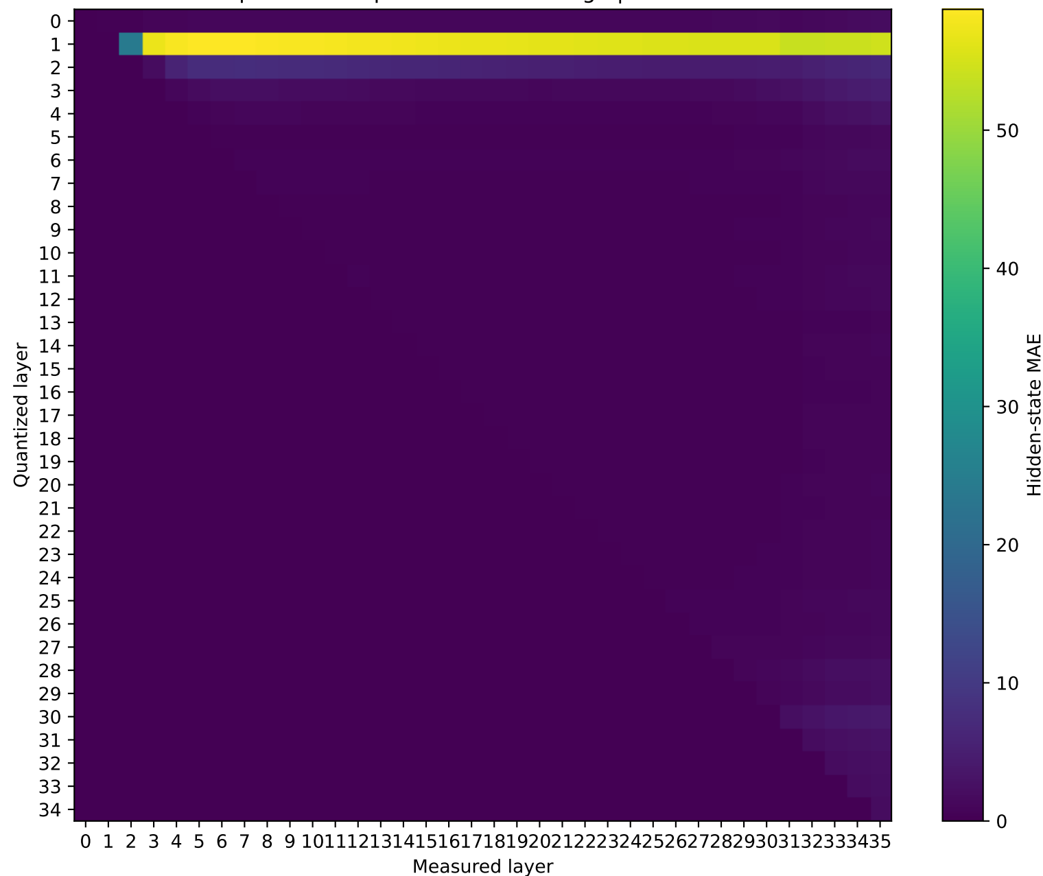
Prompt 0: MAE representation damage | float16 \rightarrow int4
