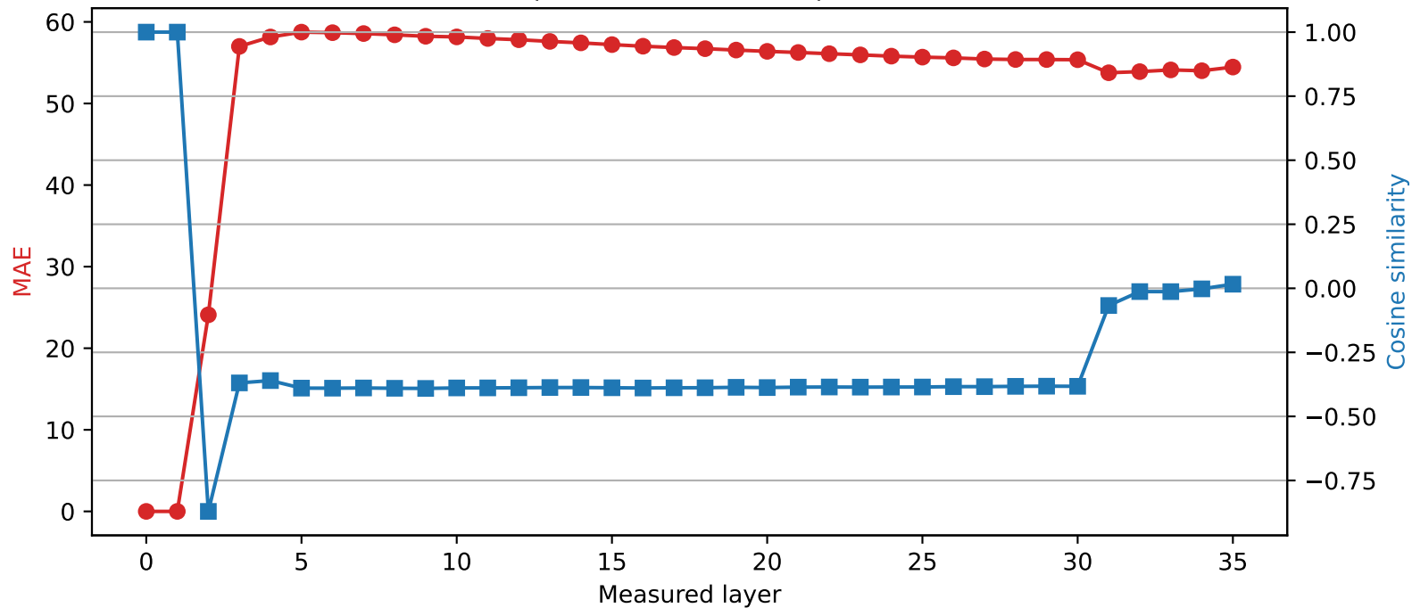
Qwen2.5-3B | Quantized layer 1 | float16 \rightarrow int4
