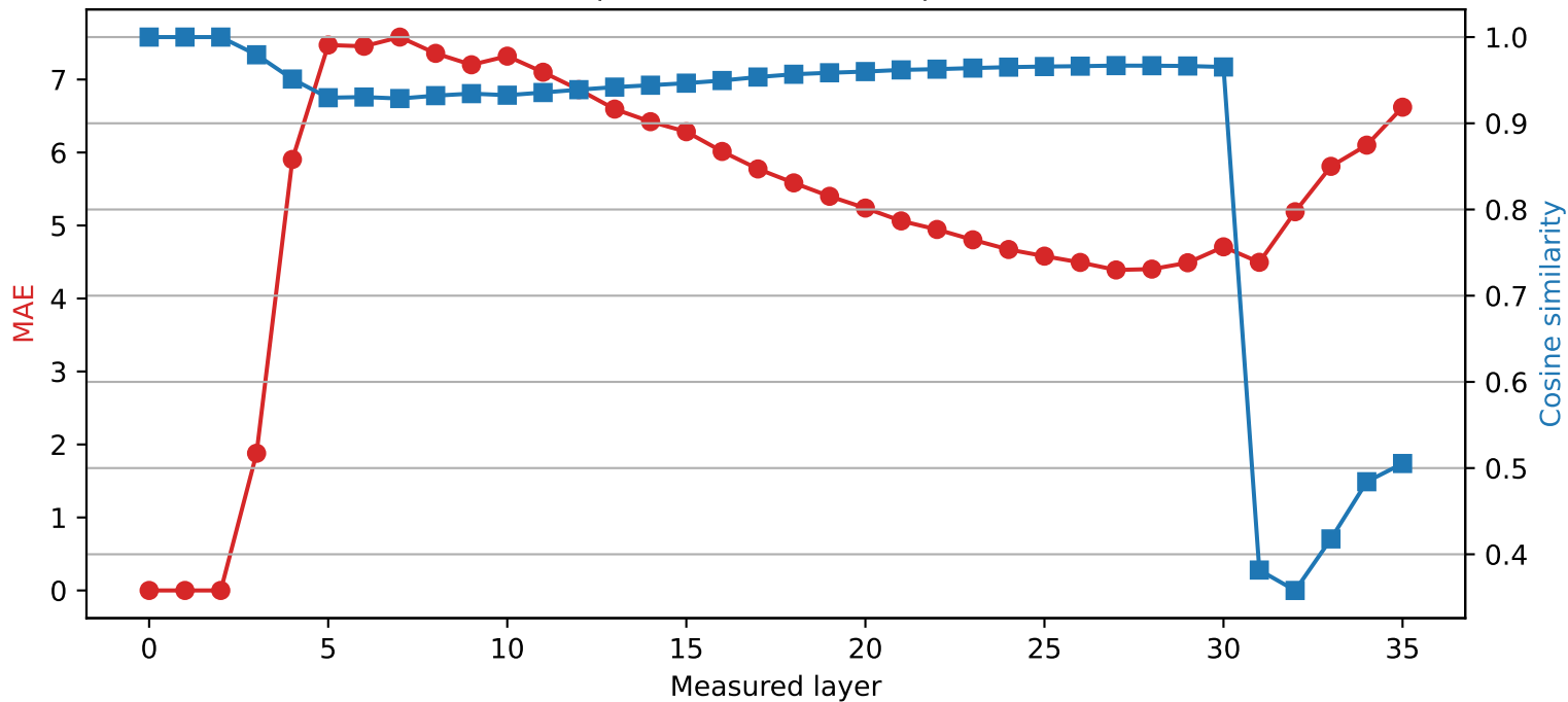
Qwen2.5-3B | Quantized layer 2 | float16 → int4
