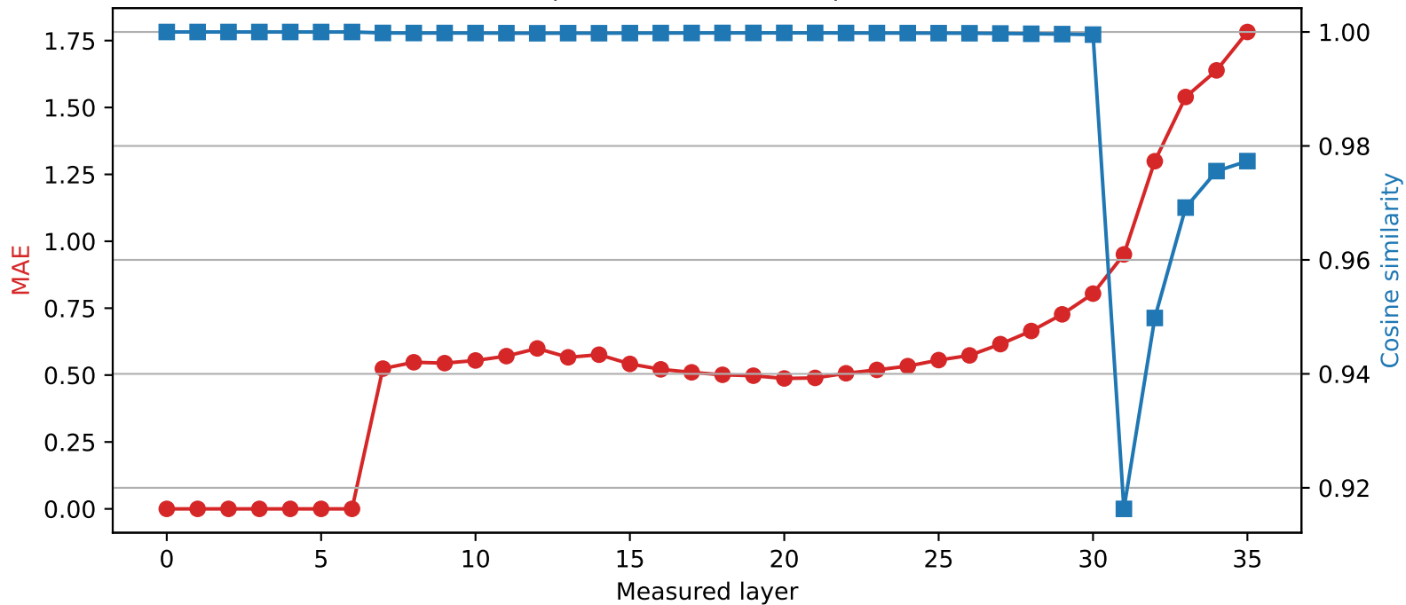
Qwen2.5-3B | Quantized layer 6 | float16 \rightarrow int4
