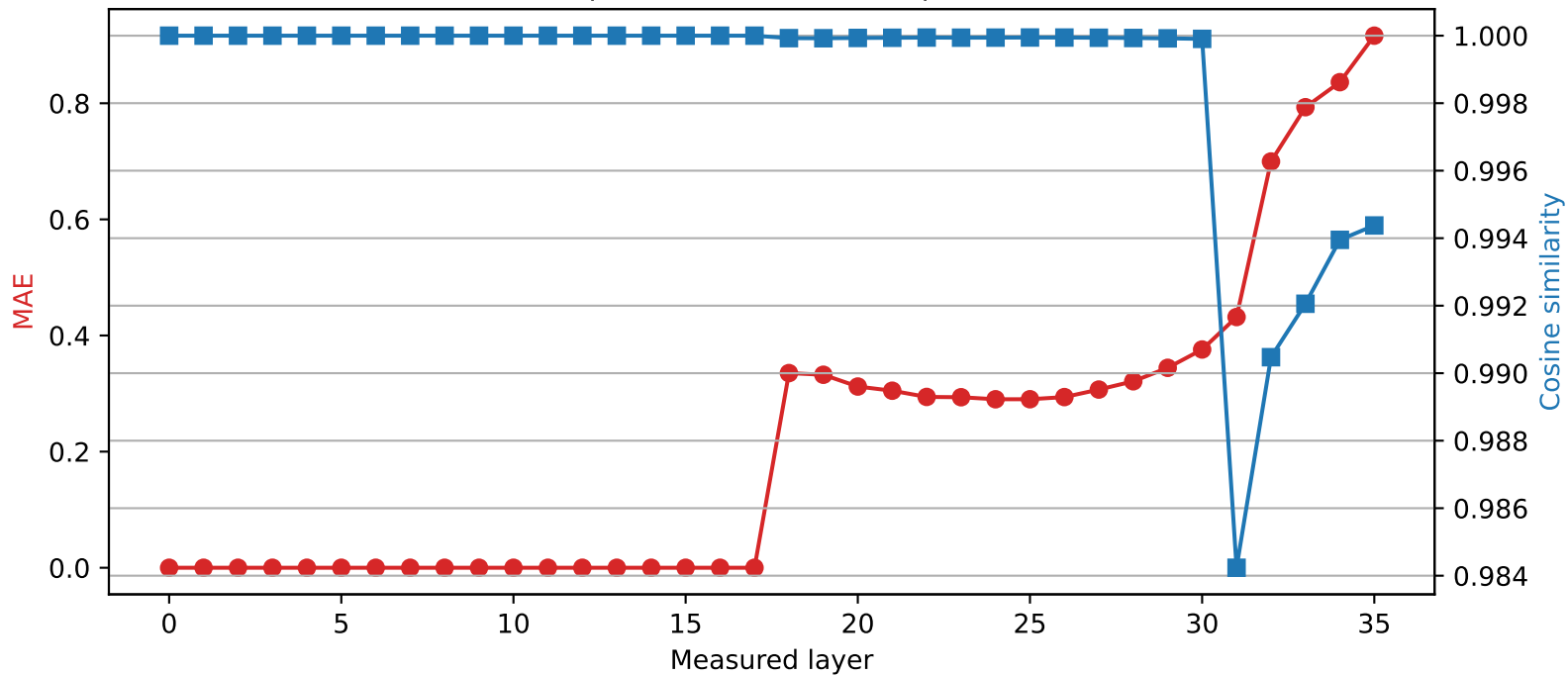
Qwen2.5-3B | Quantized layer 17 | float16 \rightarrow int4
