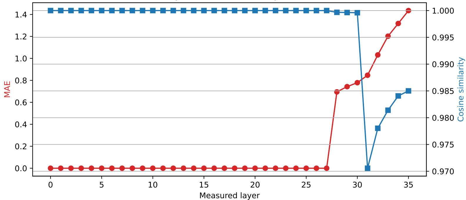
Qwen2.5-3B | Quantized layer 27 | float16 \rightarrow int4
