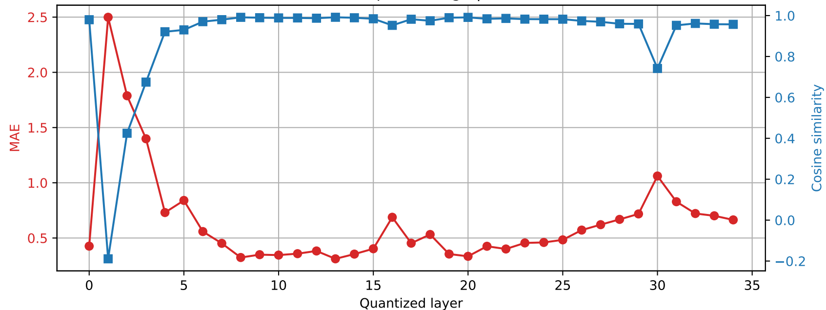
Qwen2.5-3B | Prompt 1 Final RMSNorm output damage | float16 \rightarrow int4
