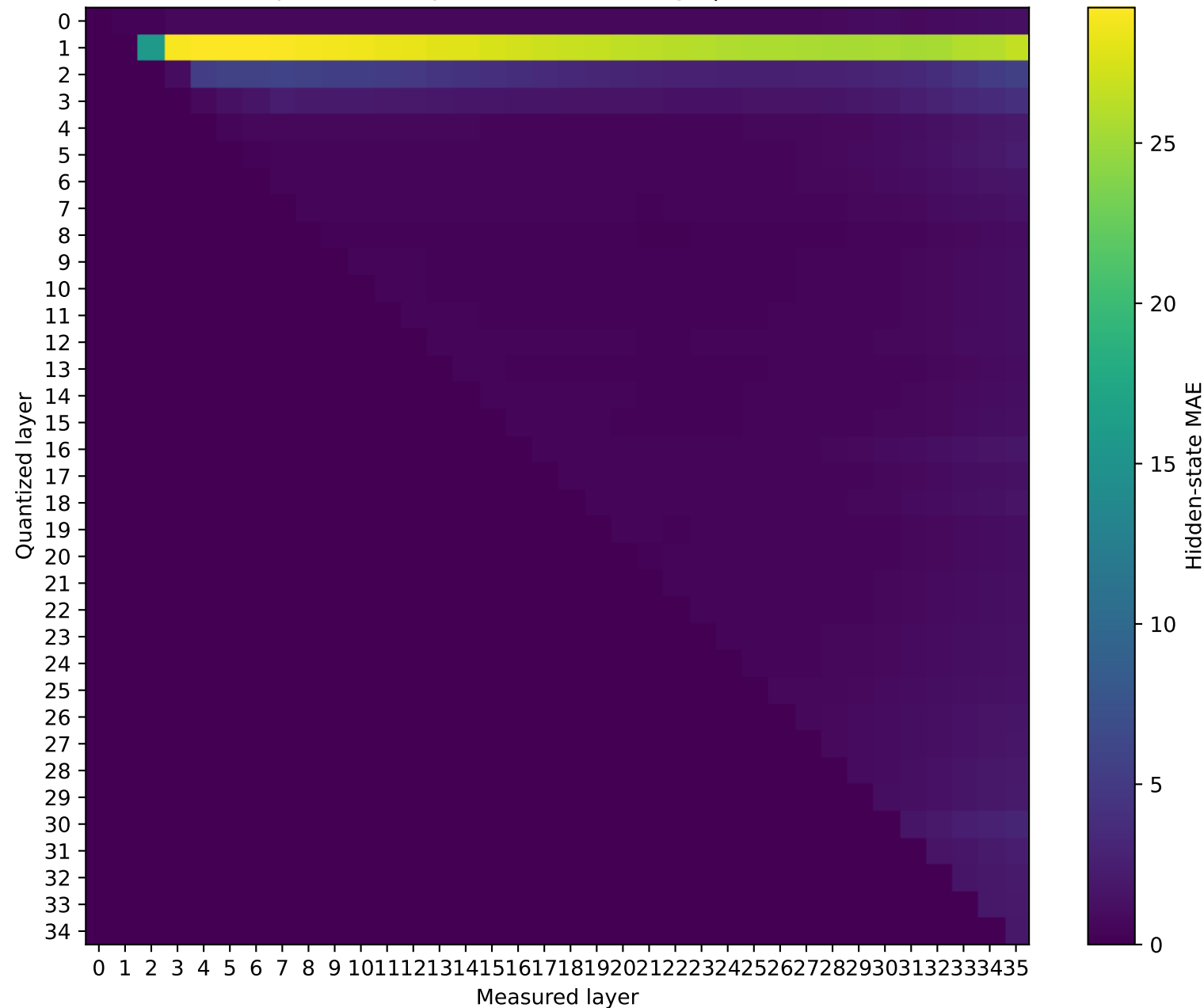
Qwen2.5-3B Prompt 1: MAE representation damage | float16 → int4
